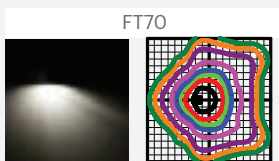
Forward Throw Optic (FT70)
