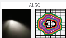
Flood Optic - AL50
