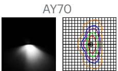
Street Optic 70°
